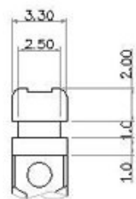
DETAIL OF LEVER
